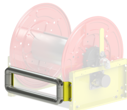
▶ LOWER HOSE GUIDE FOR FIXED GROUND INSTALLATION OR CEILING GUÍA PARA MANGUERA INFERIOR
